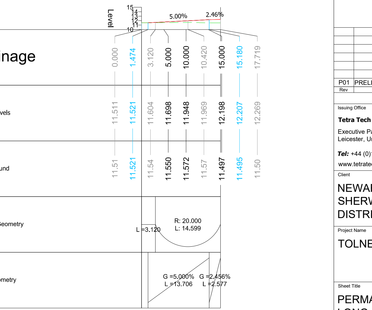
ALIGNMENT - RIVERSIDE PARK CL - LONGSECTION SCALE: H 1:500,V 1:500. DATUM: 10.000
