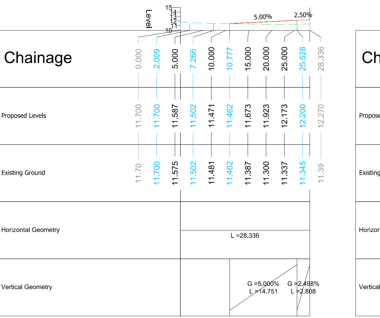
ALIGNMENT - RIVERSIDE CAR PARK CL - LONGSECTION SCALE: H 1:500,V 1:500. DATUM: 10.000
