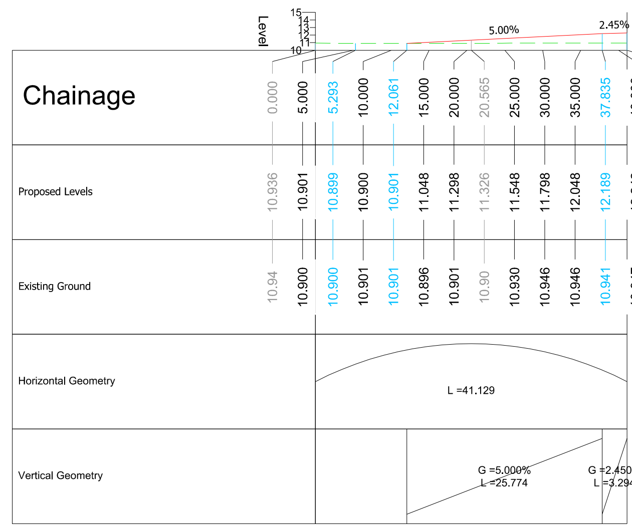
ALIGNMENT - TS3 CL - LONGSECTION SCALE: H 1:500,V 1:500. DATUM: 10.000
