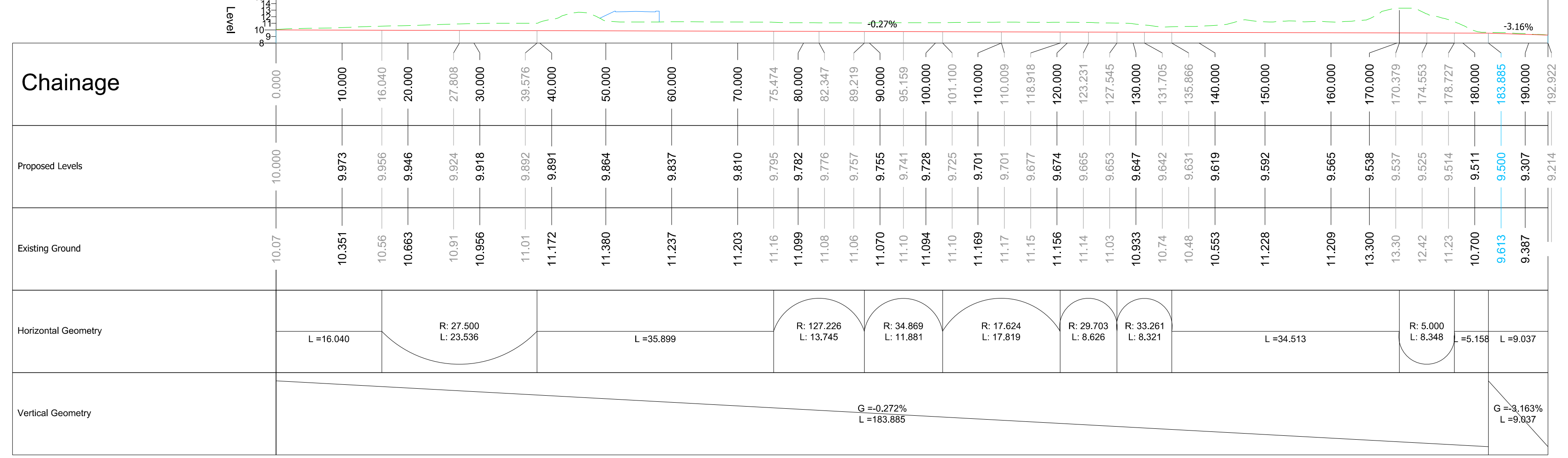
ALIGNMENT - FLOOD RELIEF CULVERT - LONGSECTION SCALE: H 1:500,V 1:500. DATUM: 8.000
