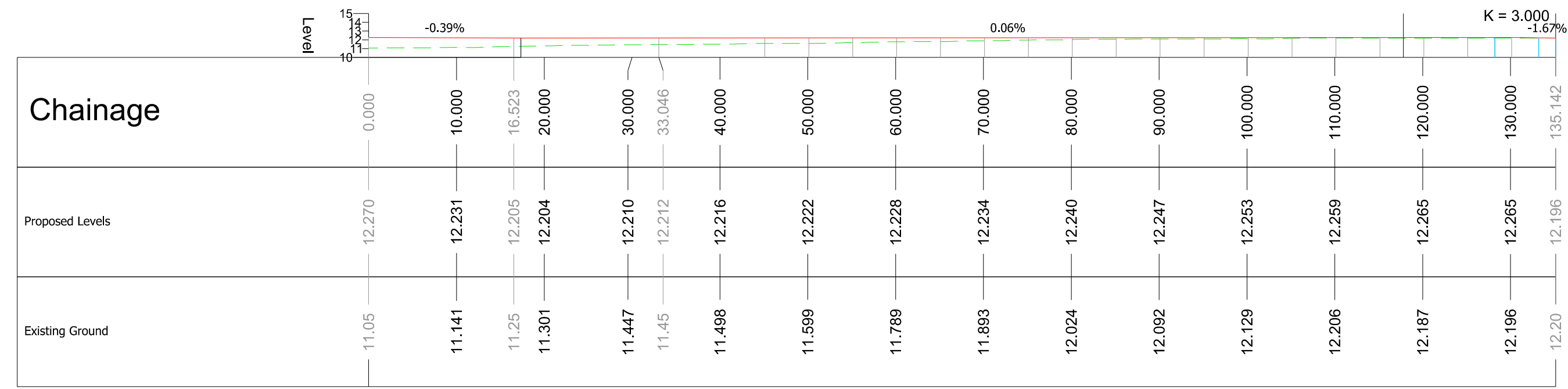
ALIGNMENT - ROAD 2 CL - LONGSECTION SCALE: H 1:500,V 1:500. DATUM: 10.000
