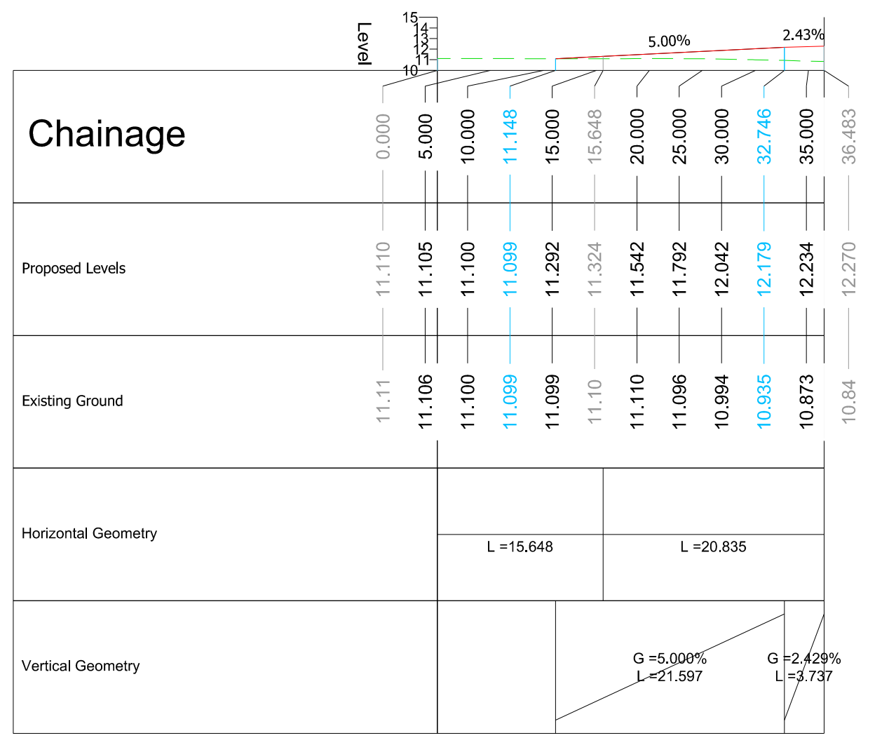
ALIGNMENT - TS2 - LONGSECTION SCALE: H 1:500,V 1:500. DATUM: 10.000
