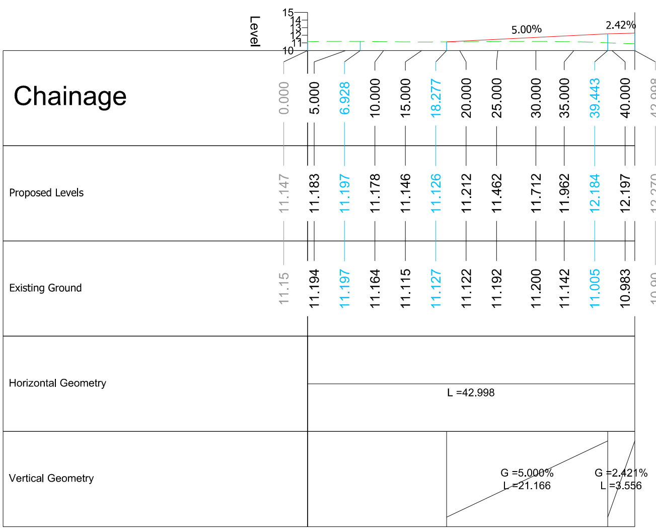
ALIGNMENT - TS1 CL - LONGSECTION SCALE: H 1:500,V 1:500. DATUM: 10.000
