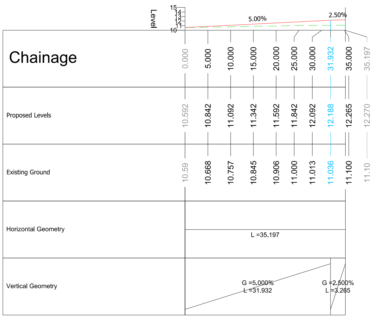
ALIGNMENT - TS4 CL - LONGSECTION SCALE: H 1:500,V 1:500. DATUM: 10.000
